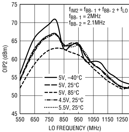
Output IP2 vs LO Frequency
