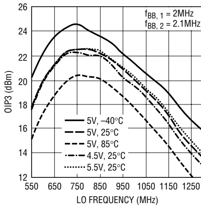
Output IP3 vs LO Frequency
