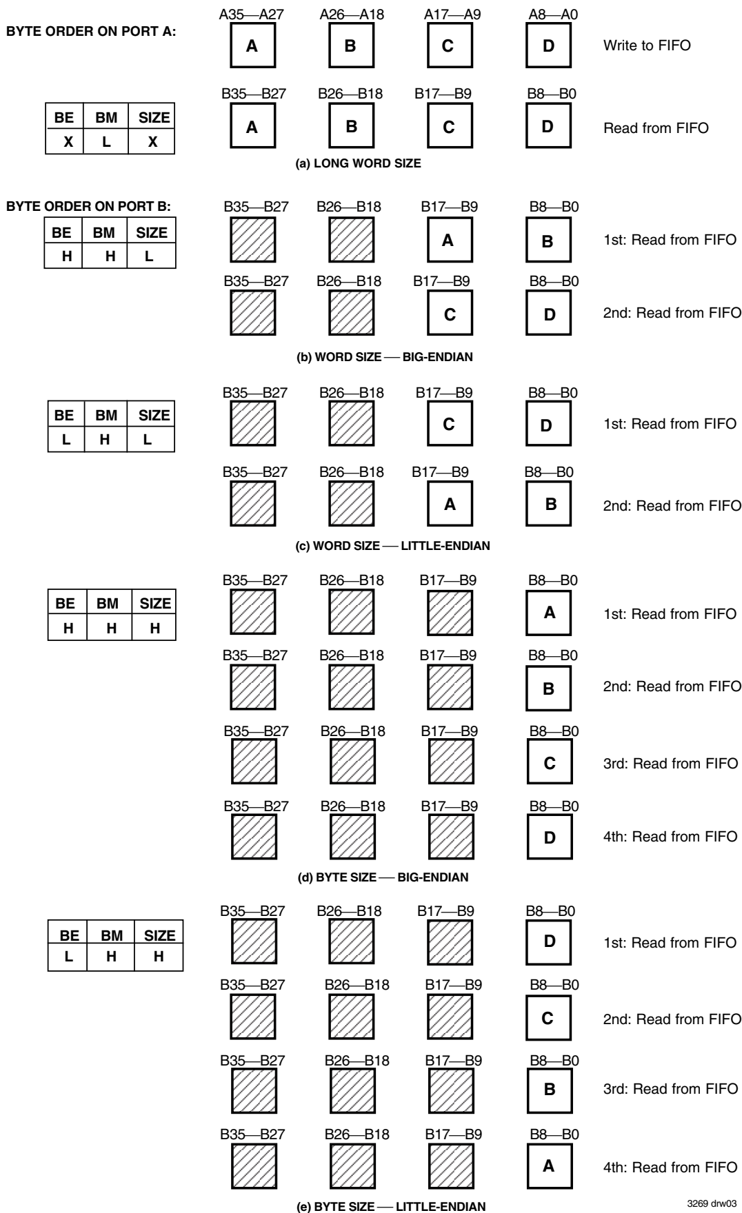
Figure 2. Bus sizing
