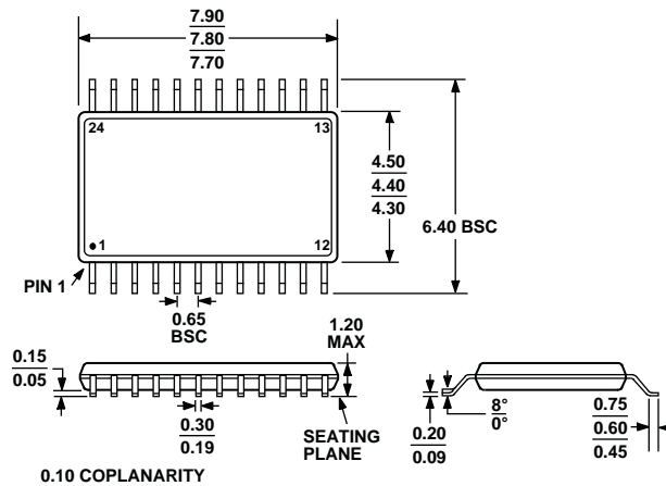
COMPLIANT TO JEDEC STANDARDS MO-153-AD Figure 41. 24-Lead Thin Shrink Small Outline Package [TSSOP] (RU-24) Dimensions shown in millimeters
