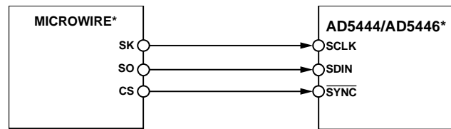
Figure 51. MICROWIRE to AD5444/AD5446 Interface
