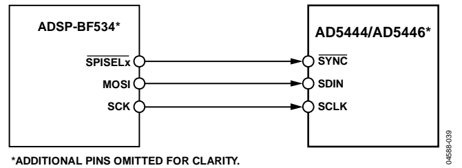
*ADDITIONAL PINS OMITTED FOR CLARITY. 04588-039 Figure 47. ADSP-BF534 to AD5444/AD5446 Interface
