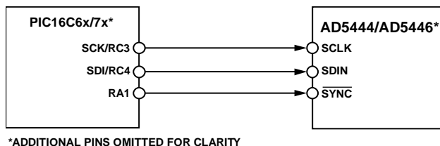
Figure 52. PIC16C6x/7x to AD5444/AD5446 Interface
