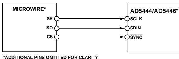
Figure 51. MICROWIRE to AD5444/AD5446 Interface
