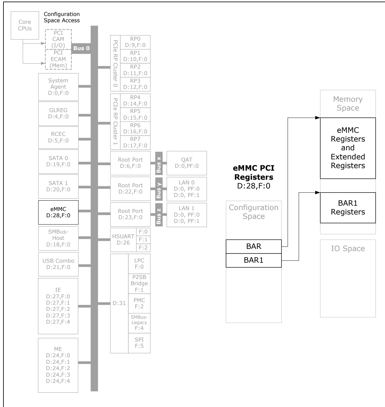
Figure 17-2. Register Map
