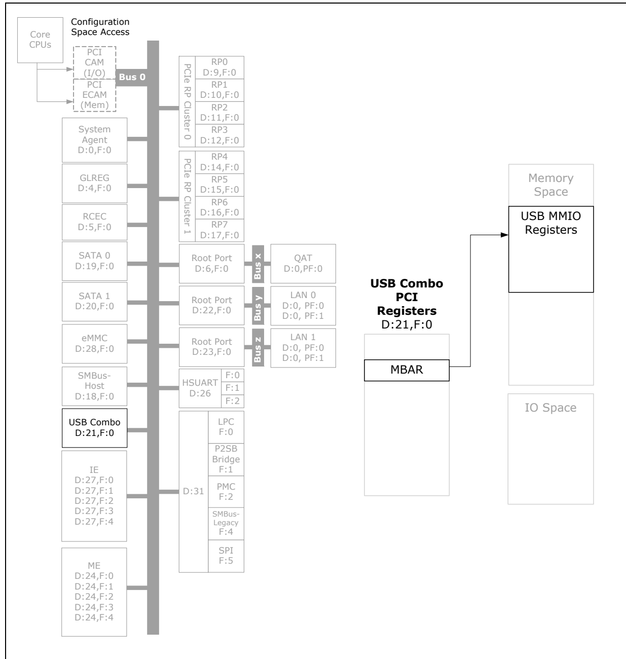
Figure 14-6. Register Map
