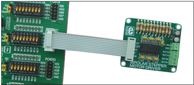
Figure 2: Bipolar Stepper Motor Driver connected to a development system
