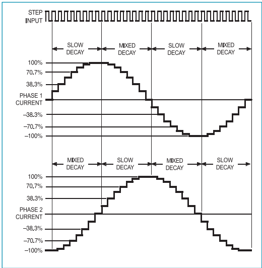
Figure 7: 8 Microstep mode: MS1=1, MS2=1, DIR=1
