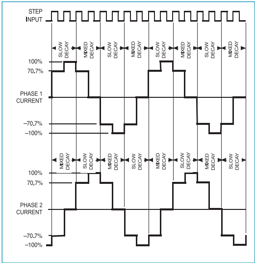
Figure 5: Half Step mode: MS1=1, MS2=0, DIR=1
