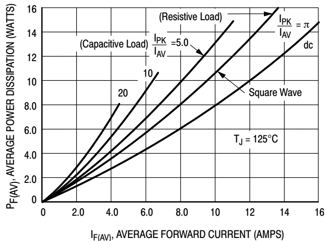
Figure 10. Power Dissipation
