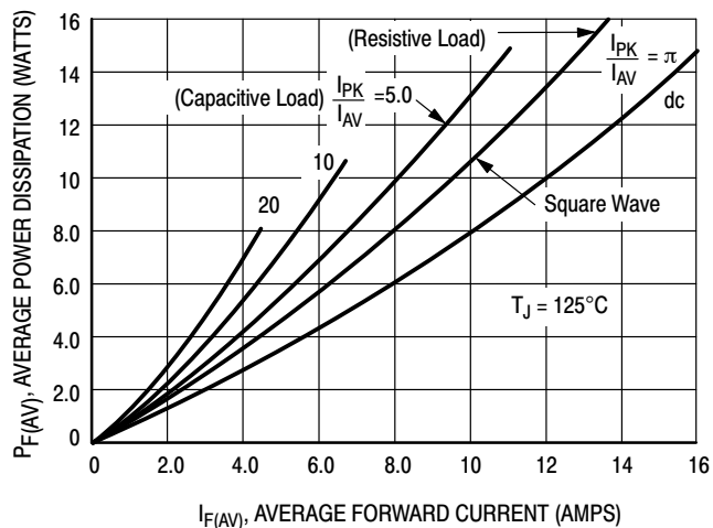
Figure 10. Power Dissipation
