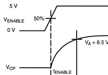
FIGURE 2. Test Circuit 2
