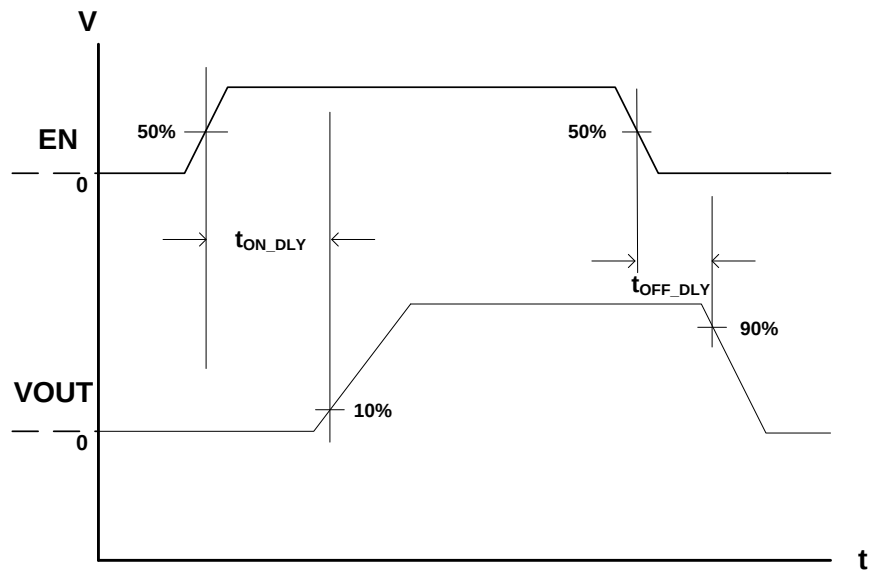
Figure 2. Turn-On/Off Delay
