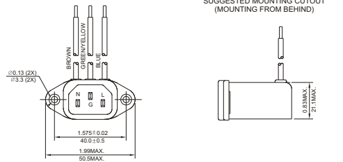
SUGGESTED MOUNTING CUTOUT (SAME AS ABOVE)
