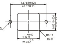
SUGGESTED MOUNTING CUTOUT
