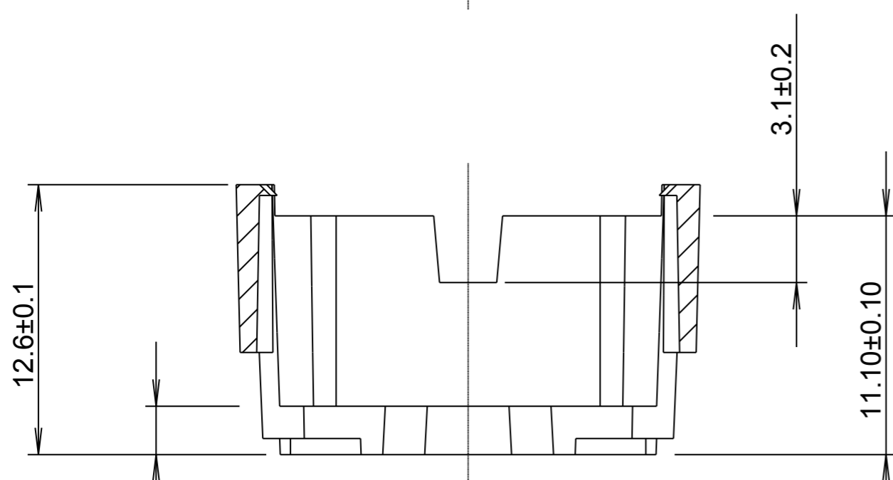
SECTION X-X
