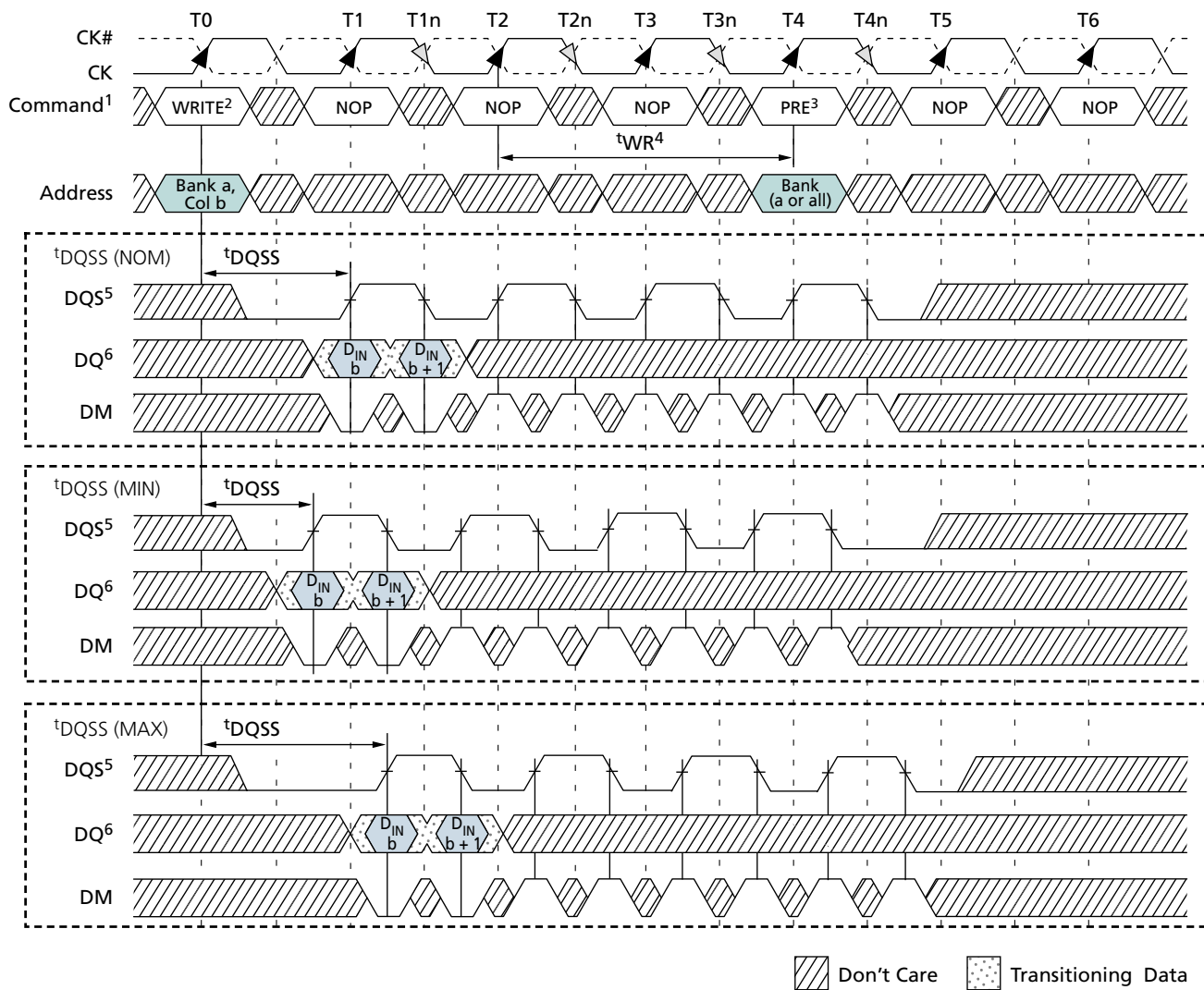
Figure 44: WRITE-to-PRECHARGE – Interrupting
