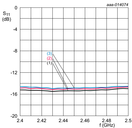
T_{\text{amb}} = 25\text{ }^{\circ}\text{C}; V_{\text{I(CTRL)}} = 0\text{ V}; \text{bypass mode} (1) V_{\text{CC}} = 3.0\text{ V} (2) V_{\text{CC}} = 3.3\text{ V} (3) V_{\text{CC}} = 3.6\text{ V}
