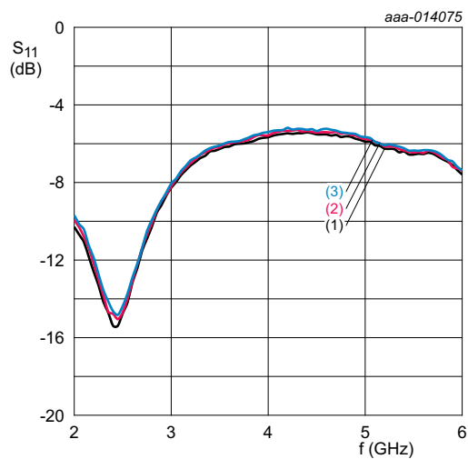
T_{\text{amb}} = 25\text{ }^{\circ}\text{C}; V_{\text{I(CTRL)}} = 0\text{ V}; \text{bypass mode} (1) V_{\text{CC}} = 3.0\text{ V} (2) V_{\text{CC}} = 3.3\text{ V} (3) V_{\text{CC}} = 3.6\text{ V}
