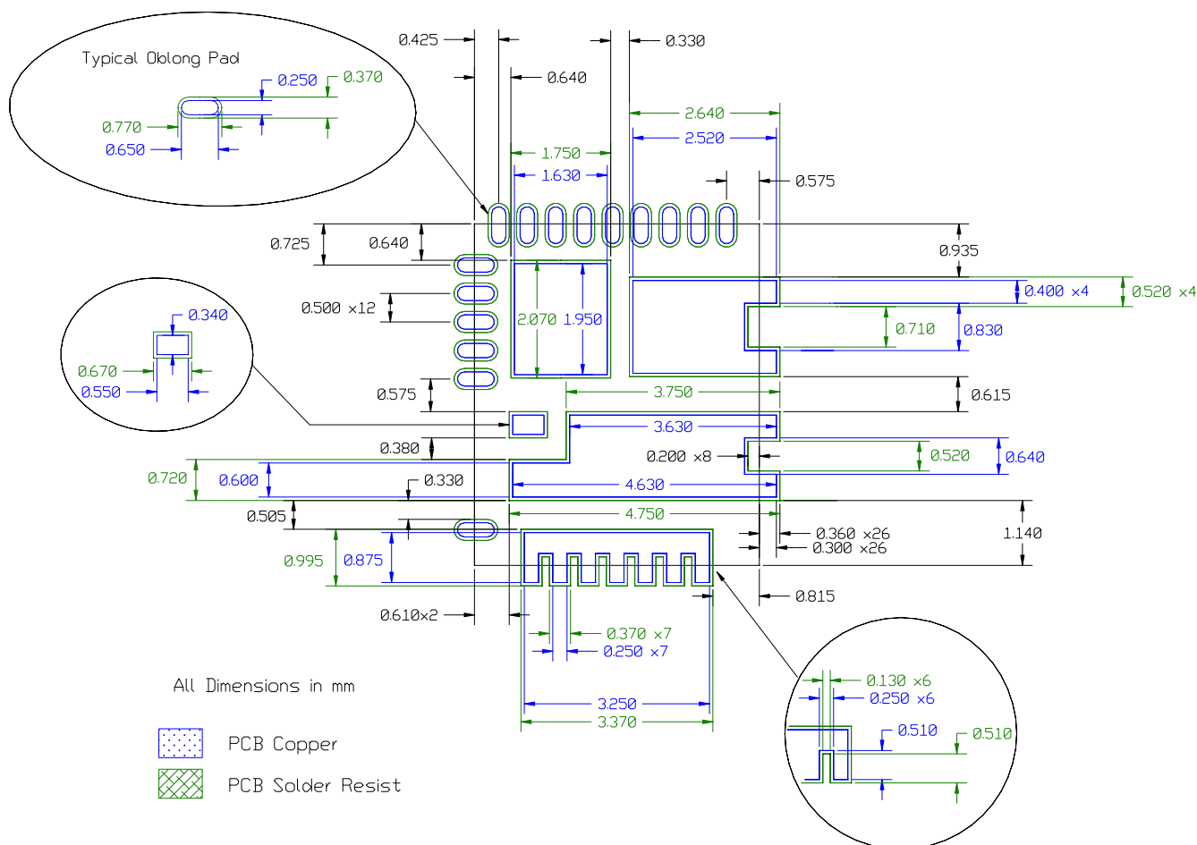
Figure 34: Solder resist
