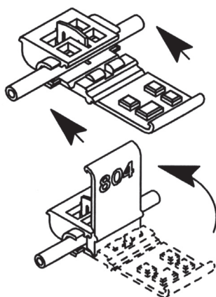
Tap Connector
