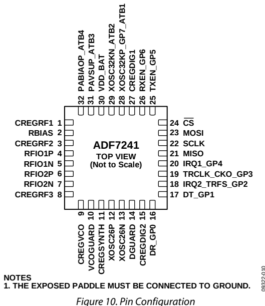
Figure 10. Pin Configuration
