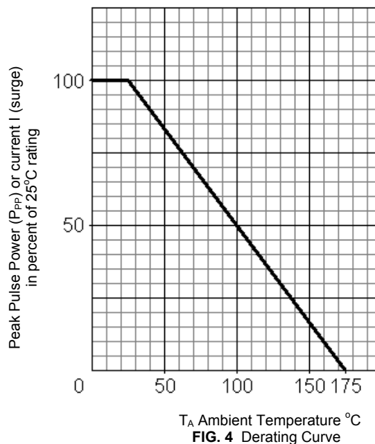
FIG. 4 Derating Curve
