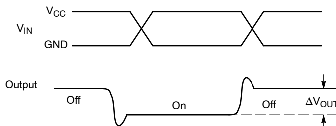
Figure 6. Charge Injection: (Q)
