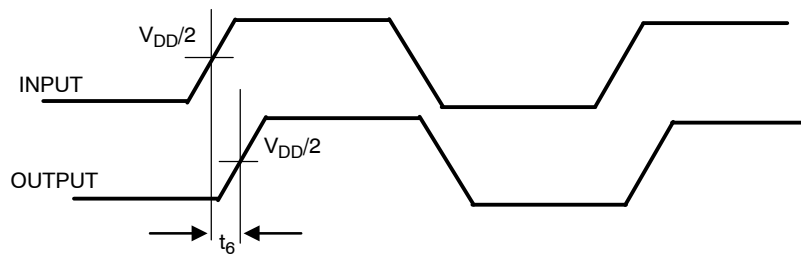
Figure 3. Switching Waveforms
