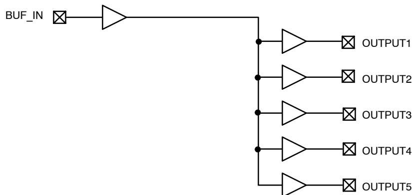
Figure 1. Block Diagram
