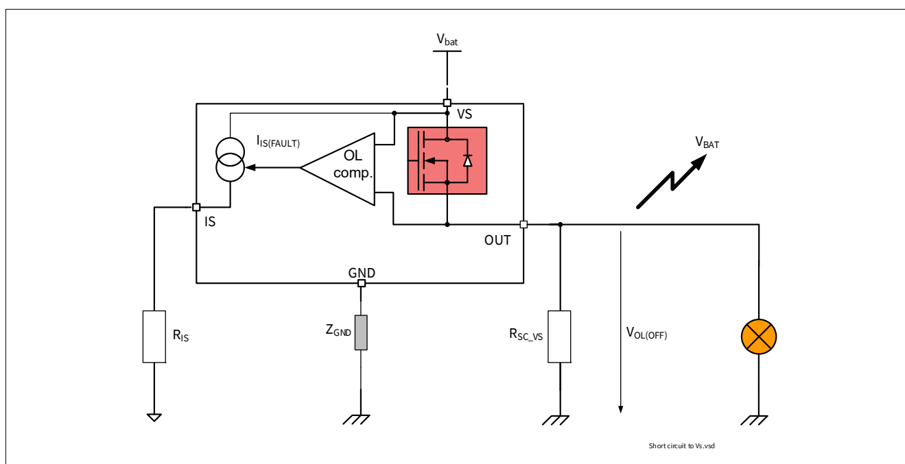
Figure 27 Short Circuit to Battery Detection in OFF Electrical Equivalent Circuit
