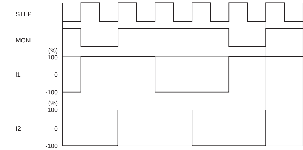
(10) Typical current waveform in each excitation mode 2-phase excitation (CW mode)
