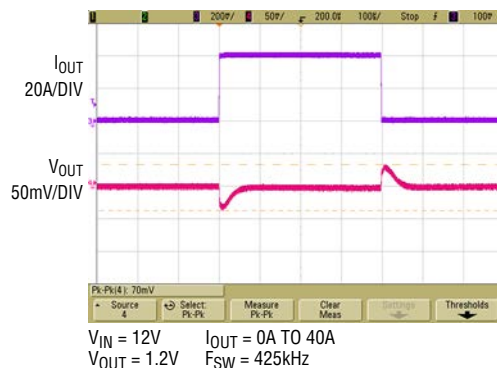
Figure 5. Load Transient Waveform DC1740A-A
