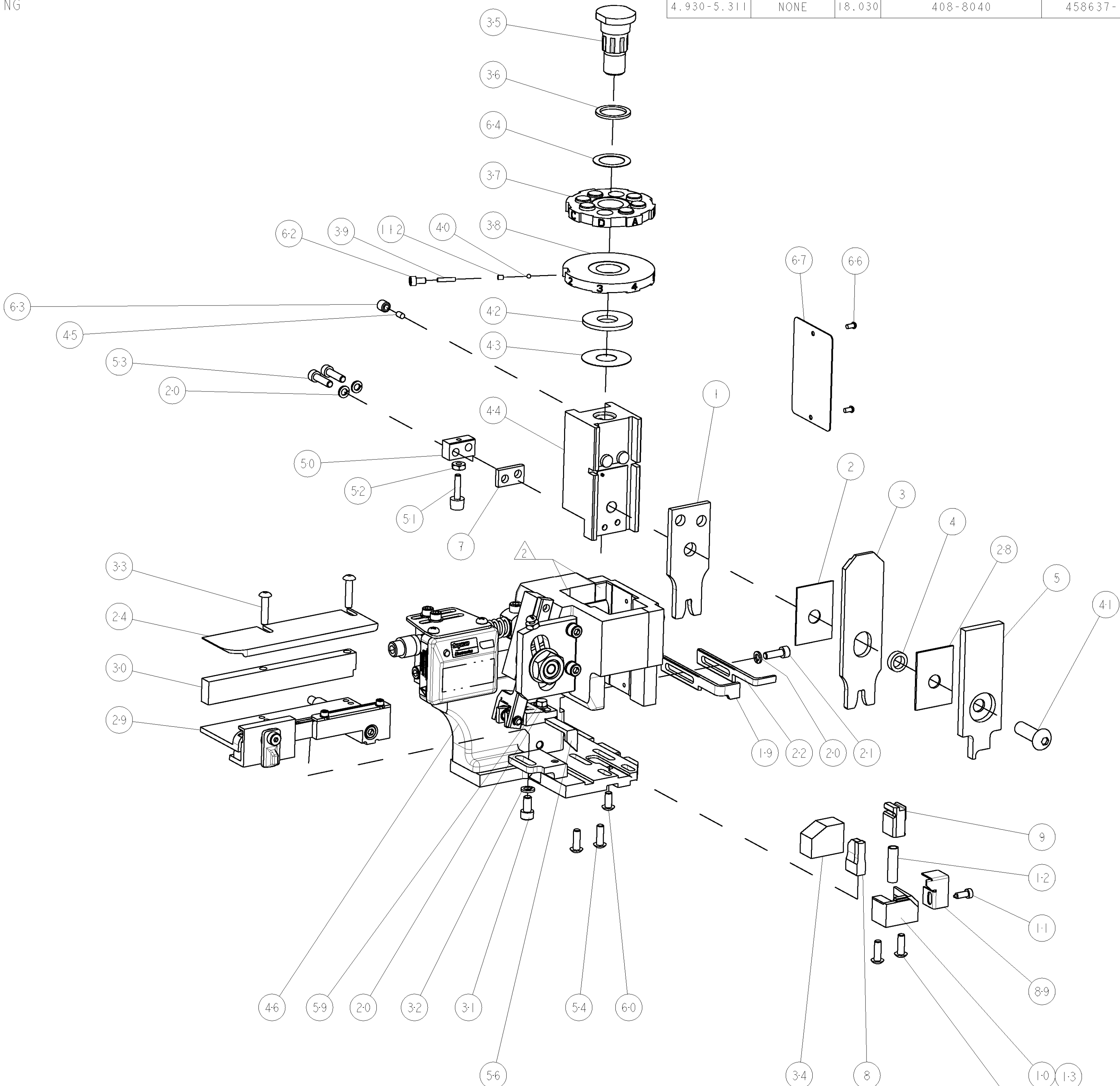
AMP-O-LECTRIC TERM GUARD
