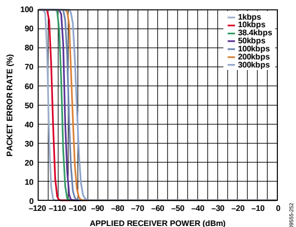
Figure 33. Packet Error Rate vs. RF Input Power and Data Rate, FSK/GFSK, 928 MHz, Preamble Length = 64 Bits, V_{DD} = 3.0 V, Temperature = 25°C
