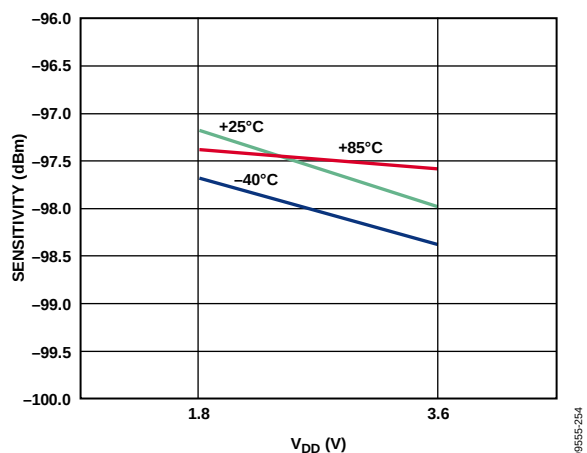
Figure 34. Receiver Sensitivity (Packet Error Rate at 1%) vs. V_{DD} , Temperature, and RF Frequency, Data Rate = 300 kbps, GFSK, Frequency Deviation = 75 kHz, IF Bandwidth = 300 kHz
