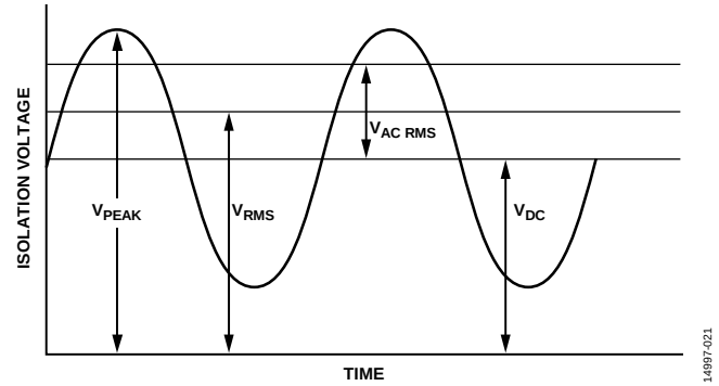
Figure 21. Critical Voltage Example
