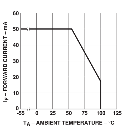
Figure 1. Forward current vs. ambient temperature.
