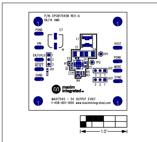
Figure 12. MAX17545 5V Output EV Kit Component Placement Guide—Component Side
