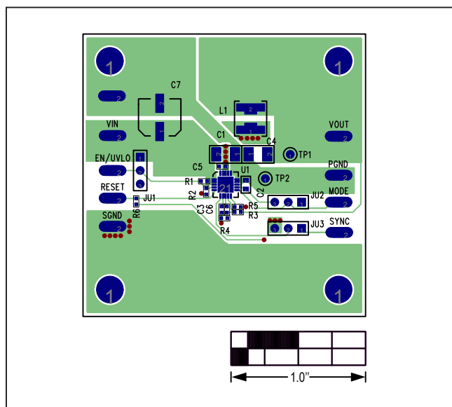
Figure 13. MAX17545 5V Output EV Kit Component Side PCB layout
