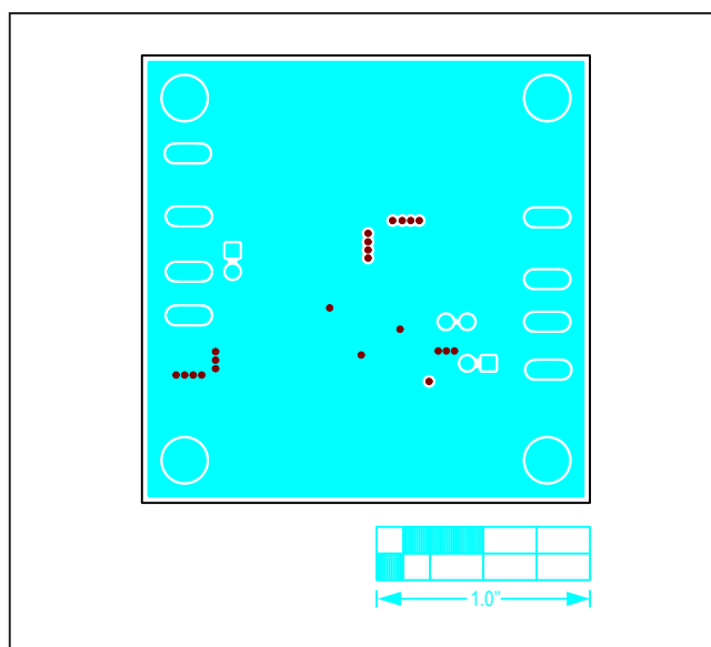
Figure 14. MAX17545 5V Output EV Kit PCB Layout—Inner Layer 1
