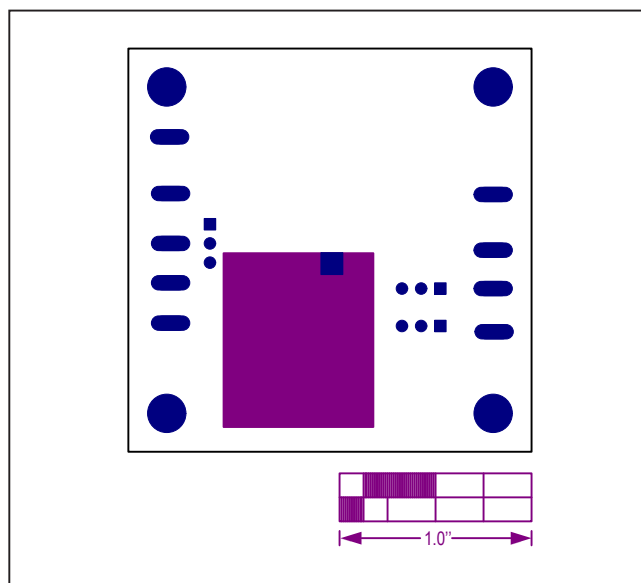
Figure 18. MAX17545 5V Output EV Kit Component Placement Guide—Bottom Solder Mask
