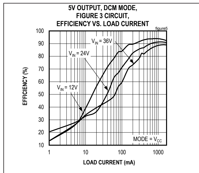
Figure 5. MAX17545 5V Output Efficiency (DCM Mode)
