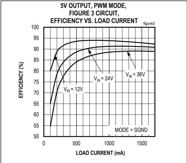
Figure 2. MAX17545 5V Output Efficiency (PWM Mode)
