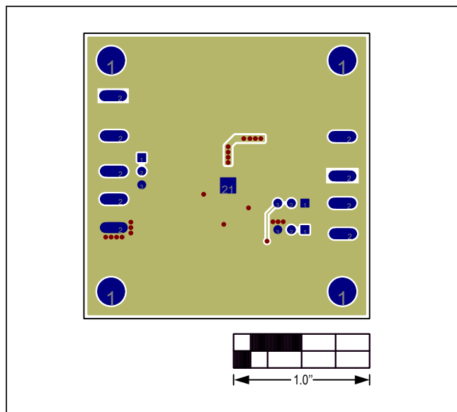
Figure 16. MAX17545 5V Output EV Kit PCB Layout—Solder Side
