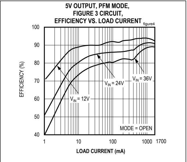
Figure 4. MAX17545 5V Output Efficiency (PFM Mode)
