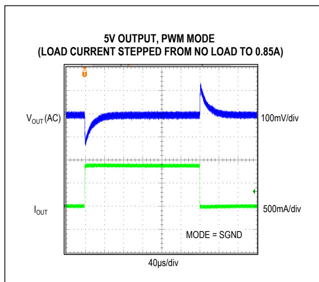
Figure 7. MAX17545 5V Output, No Load to 0.85A Load Transient (PWM Mode)
