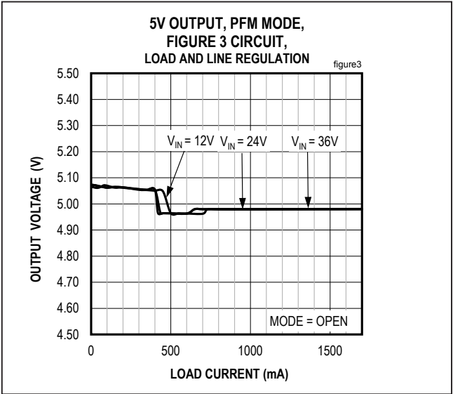
Figure 3. MAX17545 5V Output Load and Line Regulation (PFM Mode)
