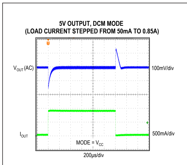
Figure 9. MAX17545 5V Output, 50mA to 0.85A Load Transient (DCM Mode)
