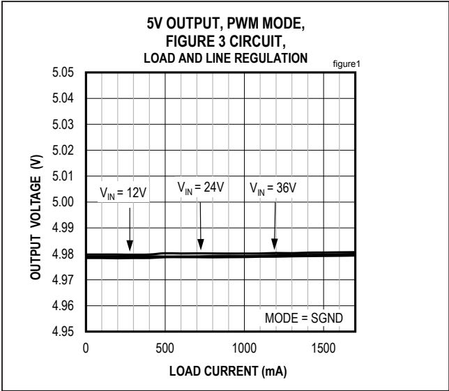
Figure 1. MAX17545 5V Output Load and Line Regulation (PWM Mode)
