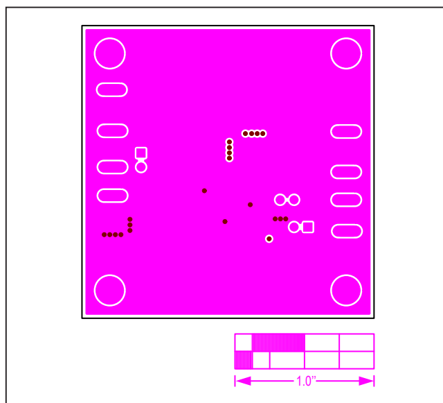
Figure 15. MAX17545 5V Output EV Kit PCB Layout—Inner Layer 2
