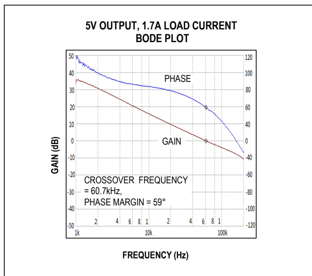
Figure 6. MAX17545 5V Output Full Load Bode Plot ( V_{IN} = 24V )
