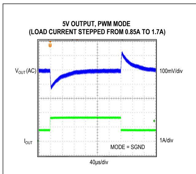
Figure 10. MAX17545 5V Output, 0.85A to 1.7A Load Transient
