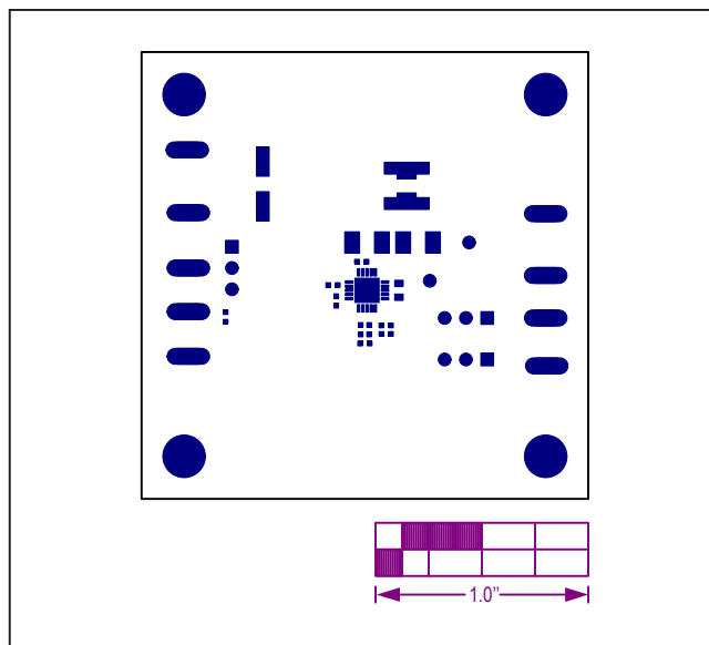
Figure 17. MAX17545 5V Output EV Kit Component Placement Guide—Top Solder Mask
