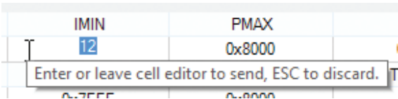
Figure 38. Cell/Register Editor
