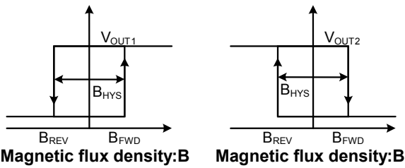
Figure 2. Output operation
