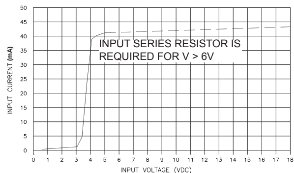
BIAS (INPUT) CURRENT VS BIAS (INPUT) VOLTAGE
