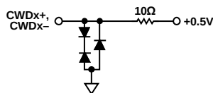
Figure 36. Equivalent CWDx± Output Circuit
