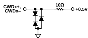
Figure 36. Equivalent CWDx± Output Circuit
