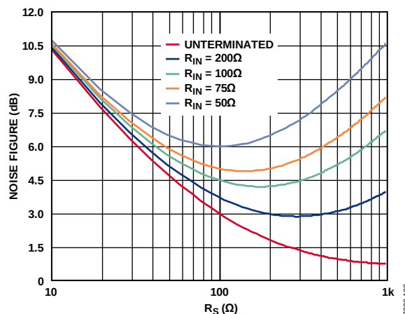
Figure 43. Noise Figure vs. R_S for Various Fixed Values of R_{IN} , Active Termination Matched Inputs, V_{GAIN} = 0.8 V
