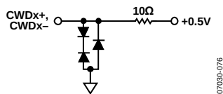
Figure 36. Equivalent CWDx± Output Circuit
