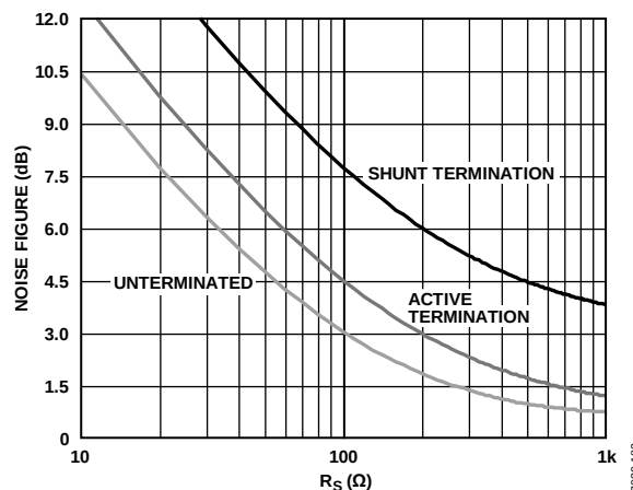
Figure 42. Noise Figure vs. R_S for Shunt Termination, Active Termination Matched, and Untermated Inputs, V_{GAIN} = 0.8 V
