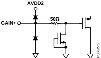
Figure 34. Equivalent GAIN+ Input Circuit
