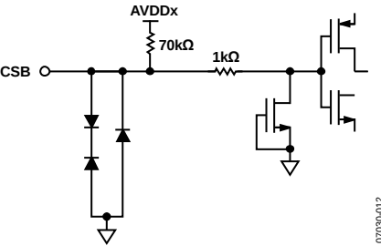
Figure 32. Equivalent CSB Input Circuit
