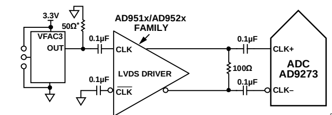
Figure 57. Differential LVDS Sample Clock
