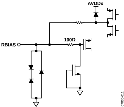
Figure 31. Equivalent RBIAS Circuit
