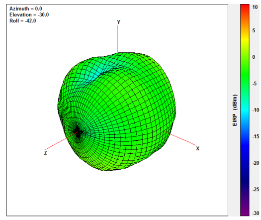
@824MHz
