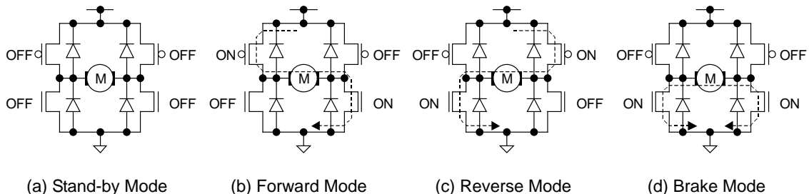
Figure 33. Four Basic Operations (Output Stage)
