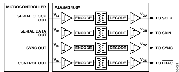
Figure 88. Isolated Interface
