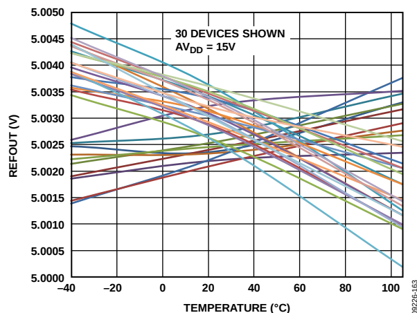
Figure 63. REFOUT vs. Temperature (When the AD5755-1 is soldered onto a PCB, the reference shifts due to thermal shock on the package. The average output voltage shift is -4\text{ mV} . Measurement of these parts after seven days shows that the outputs typically shift back 2\text{ mV} toward their initial values. This second shift is due to the relaxation of stress incurred during soldering.)
