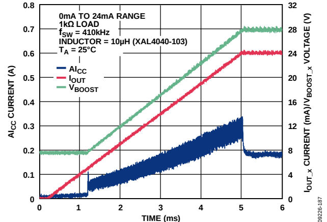
Figure 85. AI_{CC} Current vs. Time for 24 mA Step Through 1 k \Omega Load with Slew Rate Control
