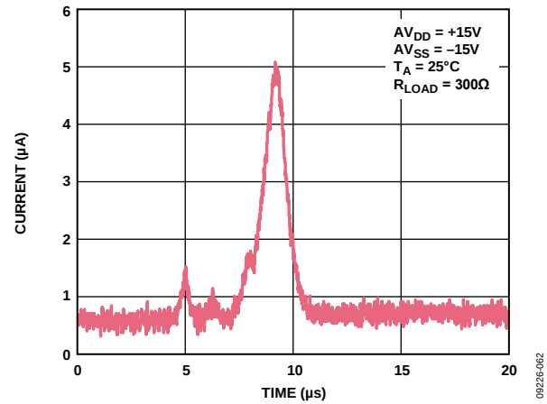
Figure 47. Output Current vs. Time on Power-Up
