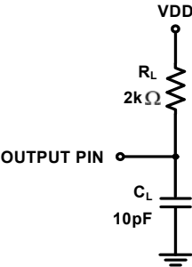
FIGURE 2. EQUIVALENT LOAD CIRCUIT FOR DIGITAL OUTPUT TESTING
