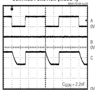
HIGH-VOLTAGE SWITCH CONTROL FUNCTION (MODE 1)
