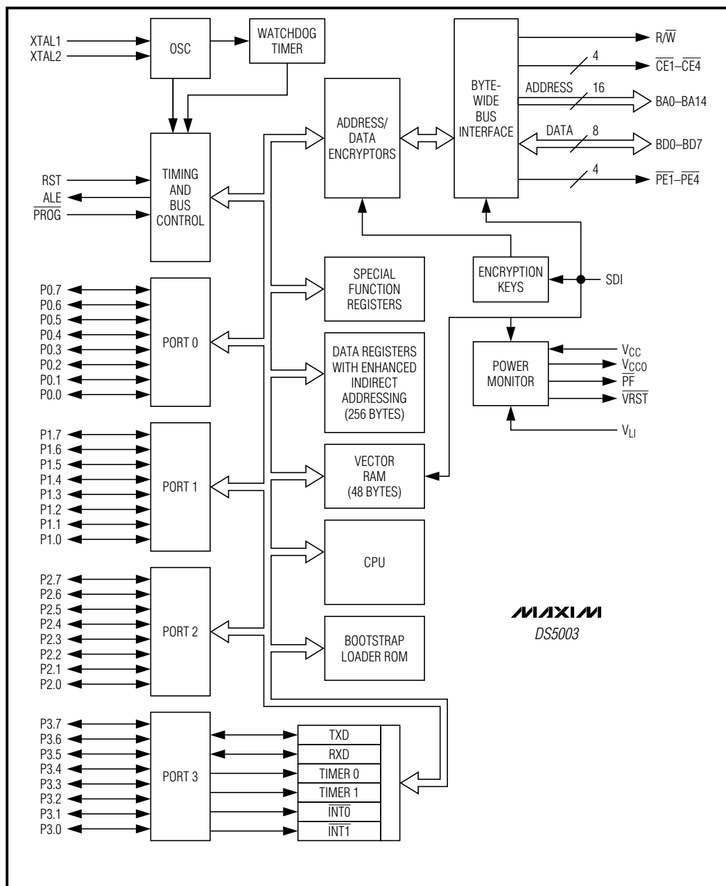
Figure 8. Block Diagram
