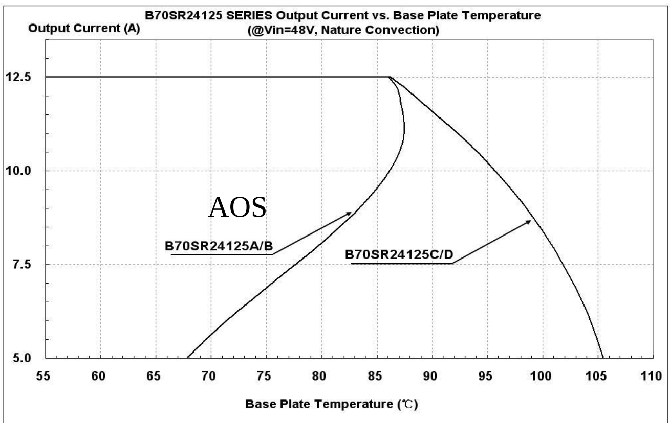
Figure 18: Output Power vs. base plate temperature @Vin=48V
