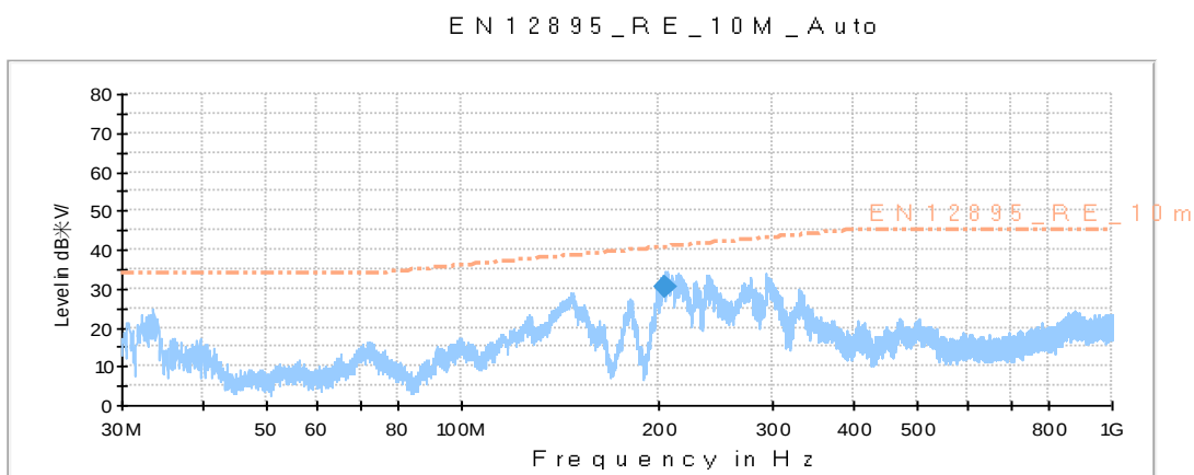
Figure 16: test result(Horizontal)
