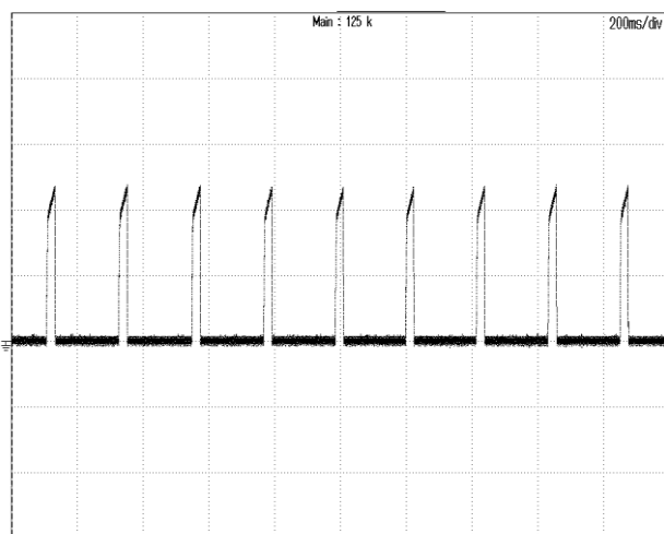
Figure 11: Output short current @ Vin=72V CH1:I o , 10A/div, 200mS/div
