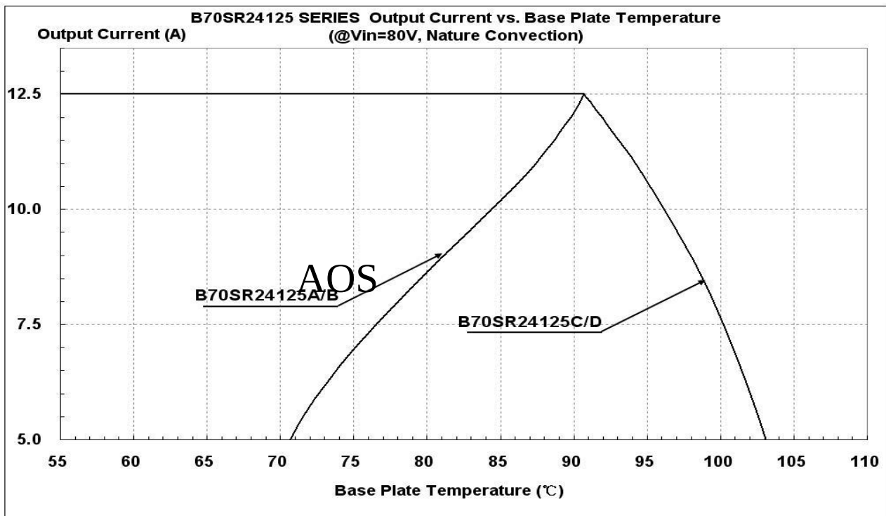
Figure 20: Output Power vs. base plate temperature @Vin=80V
