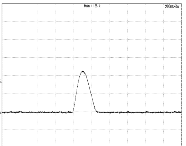
Figure 12: Inrush current @ Vin=72V CH1:I in , 2A/div, 200nS/div; Max current 4.3A, I 2t =1.5E-7 A 2 S
