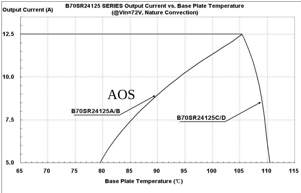
Figure 19: Output Power vs. base plate temperature @Vin=72V
