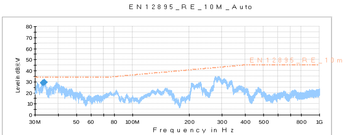
Figure 15: test result(Vertical)
