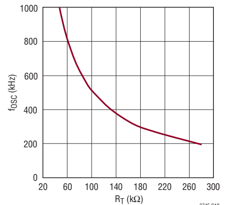
Oscillator Frequency f_{OSC} vs R_T
