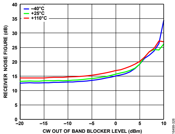
Figure 202. Receiver Noise Figure vs. CW Out of Band Blocker Level, Receiver LO = 1685 MHz, Blocker = 2085 MHz
