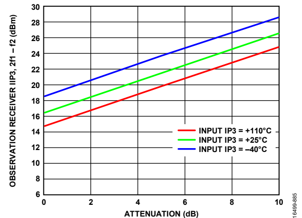
Figure 386. Observation Receiver IIP3, 2f1 – f2 vs. Attenuation, LO = 5700 MHz, Tone 1 = 5702 MHz, Tone 2 = 5822 MHz at –19 dBm Plus Attenuation
