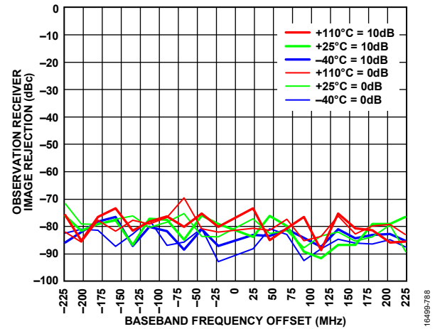
Figure 285. Observation Receiver Image Rejection vs. Baseband Frequency Offset, CW Signal Swept Across the Band, LO = 3600 MHz
