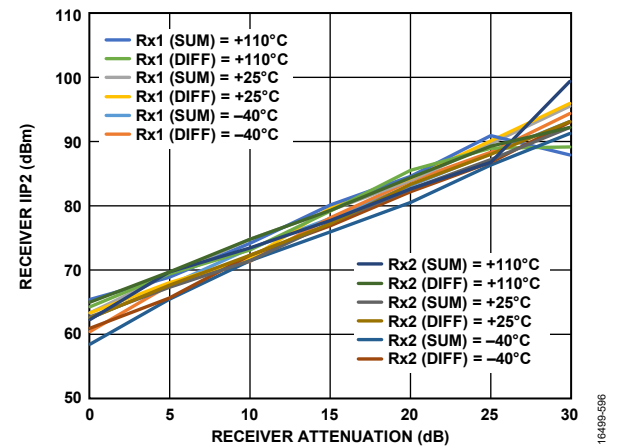
Figure 93. Receiver IIP2 vs. Receiver Attenuation, LO = 75 MHz, Tones Placed at 77 MHz and 97 MHz, -23.5 dBm Plus Attenuation
