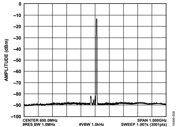
Figure 155. Amplitude vs. Frequency, Transmitter Output Spurious, Transmitter 1 = 2850 MHz, LTE = 5 MHz, Offset = 10 MHz, RMS = -12 dBFS, Temperature = 25°C
