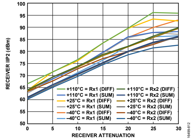
Figure 309. Receiver IIP2 vs. Receiver Attenuation, LO = 4600 MHz, Tones Placed at 4602 MHz and 4692 MHz, -21dBm Plus Attenuation
