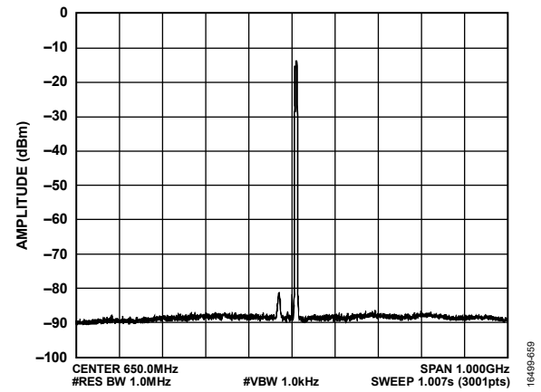
Figure 156. Amplitude vs. Frequency, Transmitter Output Spurious, Transmitter 2 = 2850 MHz, LTE = 5 MHz, Offset = 10 MHz, RMS = -12 dBFS, Temperature = 25°C
