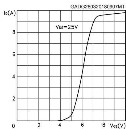
Figure 8. Transfer characteristics
