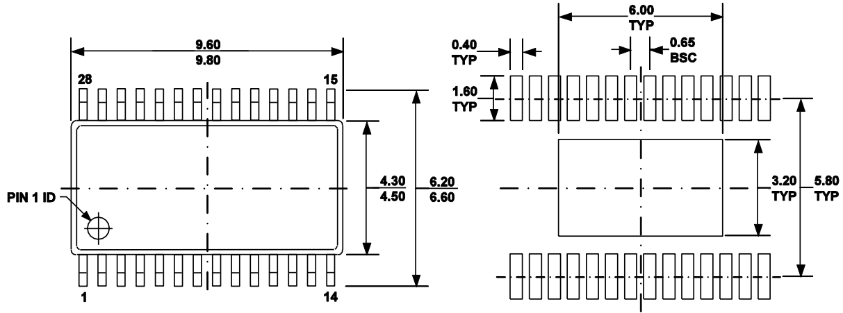
TOP VIEW
