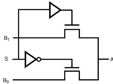
Figure 1. Logic Symbol
